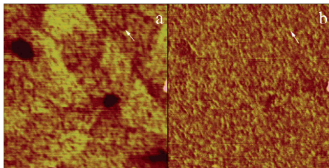
Figure 6. Phase-segregated C16- and PC-mixed SAM for determining the height of PC SAMs on Au (111) by AFM. The features (e.g., the one marked by an arrow) having lighter color in the topographic image (a) are darker in the corresponding frictional image (b).
