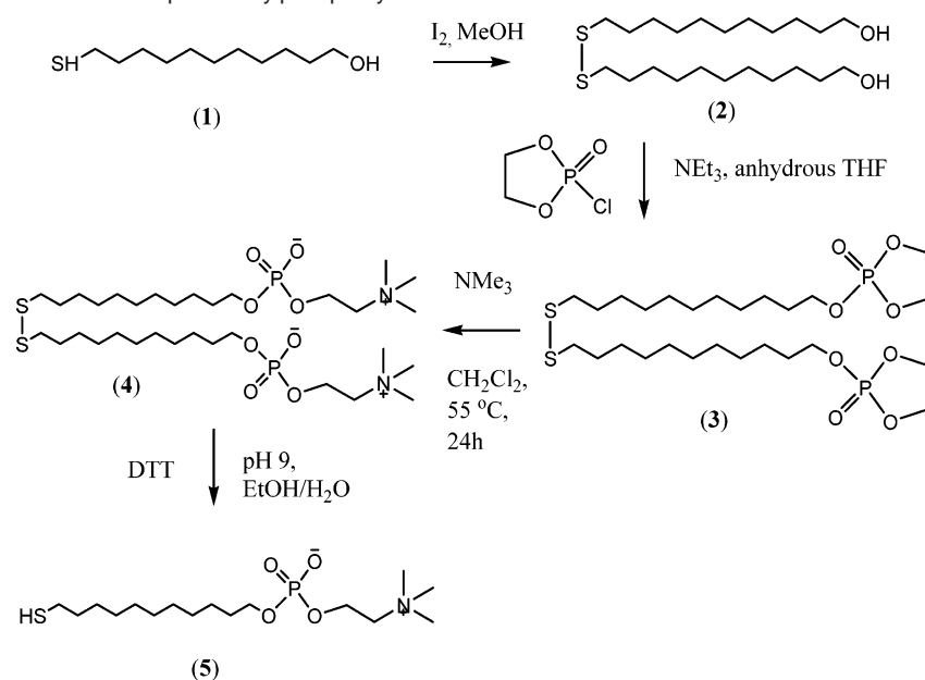
Scheme 1. Synthesis route of 11-mercaptoundecylphosphorylcholine
