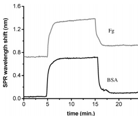
Figure 2. Adsorption of 1 mg/ml Fg and BSA in PBS buffer (0.13 M and pH 7.4) on PC SAMs from SPR. The typical SPR wavelength shifts for Fg and BSA adsorption on methyl-terminated SAMs are 16 \text{nm}^2 and 7 \text{nm}^2 , 33 respectively; 1 nm wavelength shift in SPR is equivalent to 0.15 \text{mg}/\text{m}^2 adsorbed proteins.
