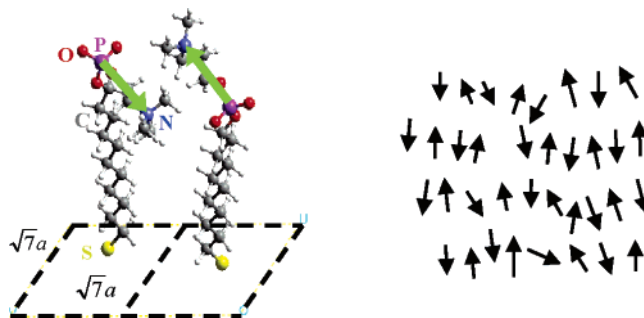
Figure 4. (a) Molecular configuration of PC SAMs from molecular simulations and (b) antiparallel orientation of PC headgroups for dipole minimization.
