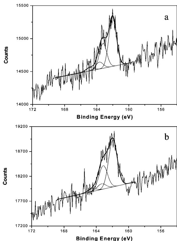
Figure 1. High-resolution spectra of the S_{2p} region from XPS for 11-mercaptopundecylphosphorylcholine SAMs prepared from a solution at (a) acidic and (b) pH 10. The peaks were fit using two S_{2p} doublets with 2:1 area ratio and splitting of 1.2 eV. The high-resolution sulfur data show up to 89% sulfur species at 162 eV, indicating that the majority of sulfur species is bound to the gold surface.
