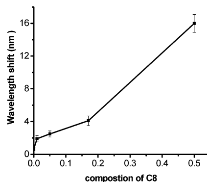
Figure 3. Fg adsorption on mixed C8 and PC SAMs from PBS buffer. With the increase of C8 composition, Fg adsorption increases.
